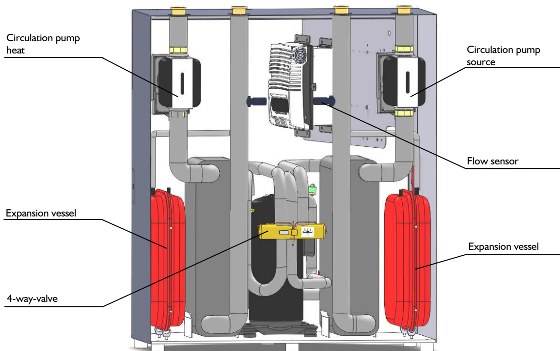
Fig. : Rear view open - perspective
