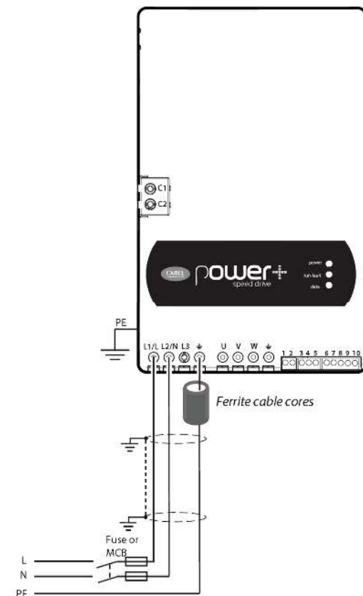
Fig.: Connecting of PSD10122** and PSD10162** Inverter
