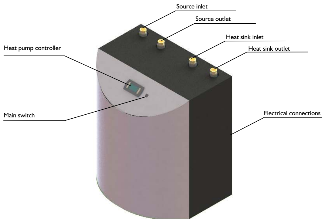
Fig. : Front view - perspective
