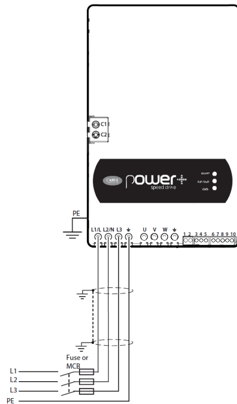
Fig.: Connecting of PSD10244 Inverter
