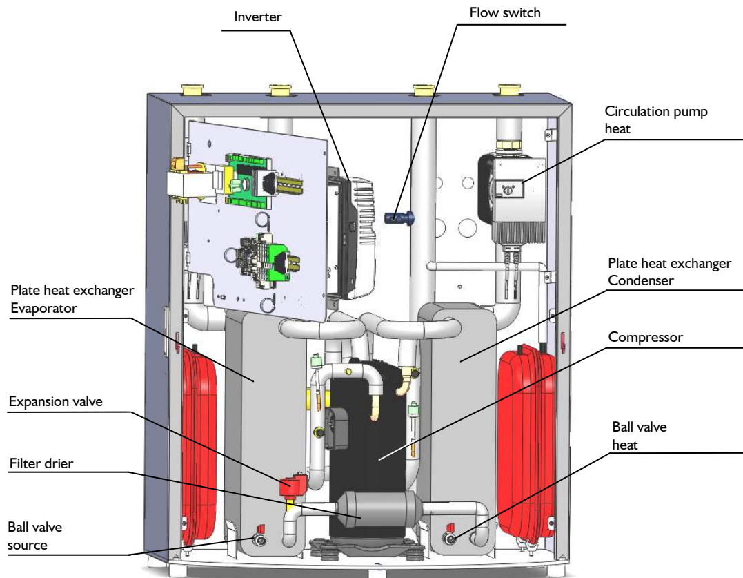
Fig. : Front view open - perspective
